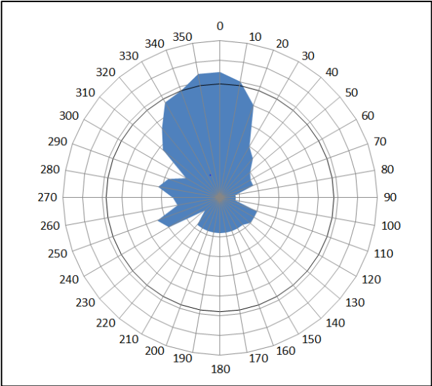
Figure 3 - XZ radiation pattern with -3dB line for calculating beam width
