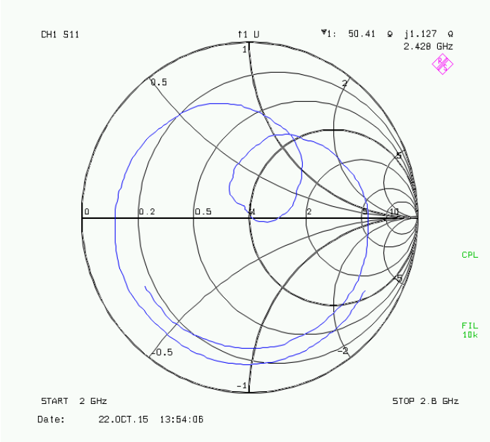
Figure 2 - Smith Chart
