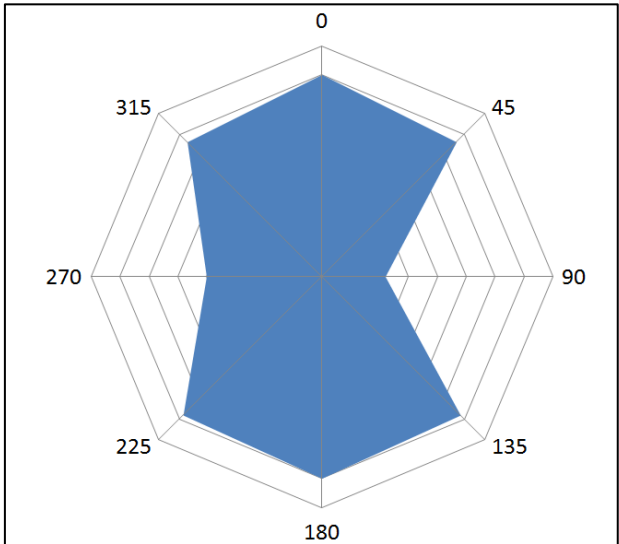
Figure 5 - XY radiation pattern
