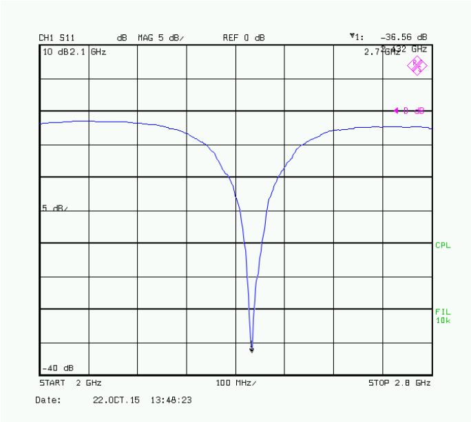
Figure 1 - Power reflection S11 (dB) vs frequency (GHz)
