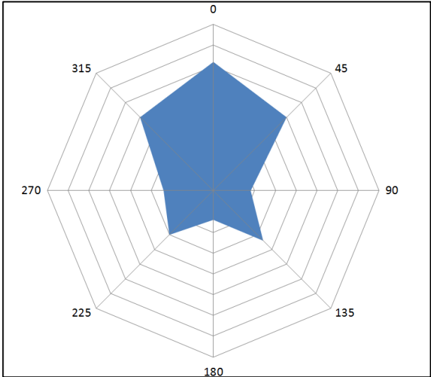
Figure 4 - YZ radiation pattern
